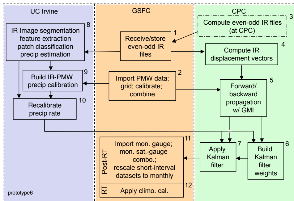
Fig. 2. High-level block diagram illustrating the major processing modules and data flows in IMERG. The blocks are organized by institution to indicate heritage, but the final code package will be an integrated system. The numbers on the blocks are for reference in Section 5. Box 3 is computed at CPC as an integral part of IMERG.
