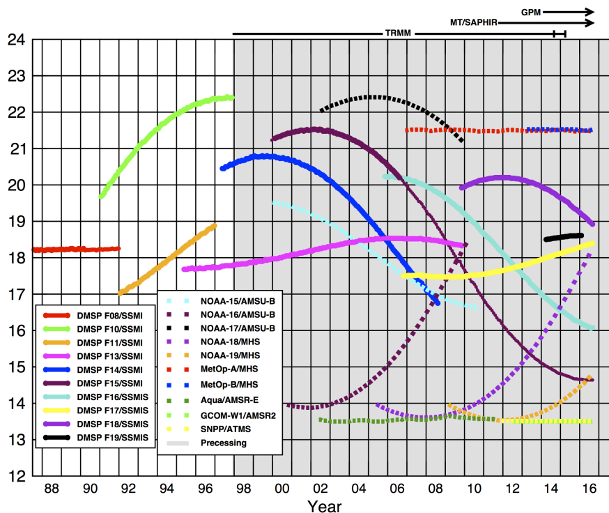
Fig. 1 PMW sensor Equator-crossing times for 12-24 Local Time (LT; 00-12 LT is the same) for the modern PMW sensor era. These are all ascending passes, except F08 is descending. Shading indicates that the precessing TRMM, Megha-Tropiques, and GPM cover all times of day. [Image by Eric Nelkin (SSAI), 22 September 2016; current version at http://precip.gsfc.nasa.gov/times_allsat.jpg .]
