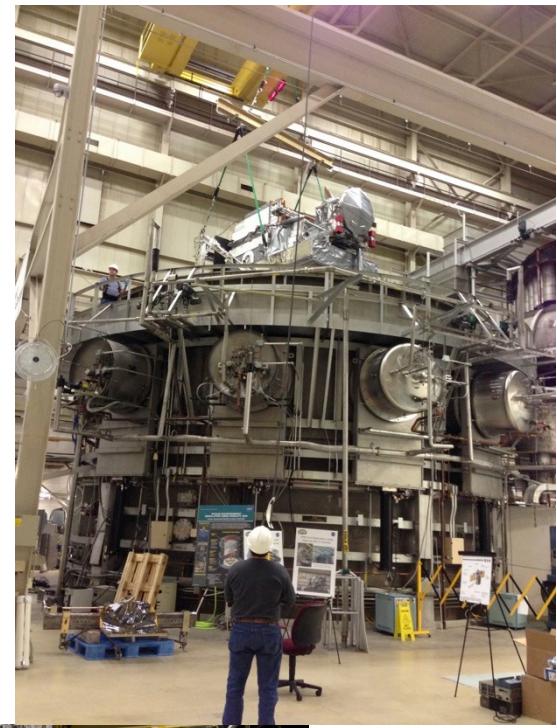
Thermal Vacuum
