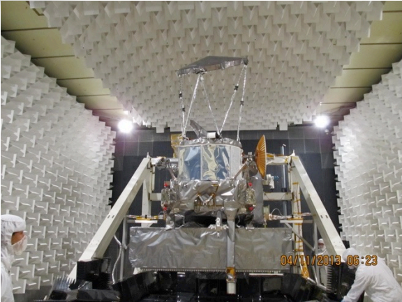
Electromagnetic Compatibility/Interference
