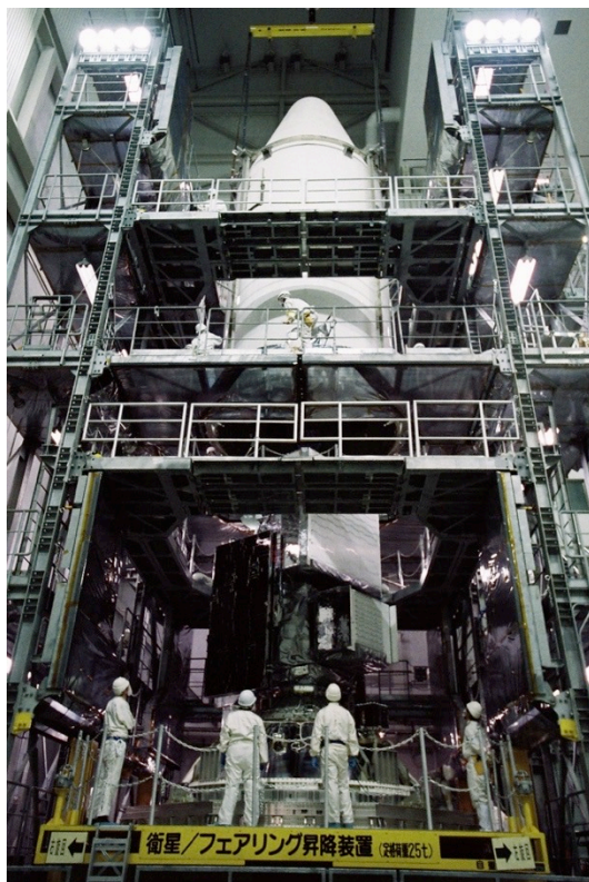
GPM Spacecraft Encapsulation in H-IIA Rocket
